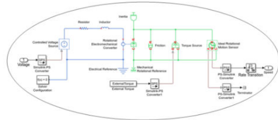
Components of 'Plant' Model block (Masked Model)
